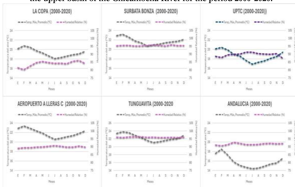
Figure 4. Behavior of maximum relative humidity and maximum temperature in the upper basin of the Chicamocha River for the period 2000-2020.
